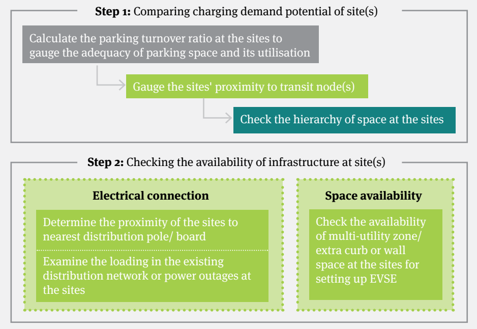
FIGURE 11: SITE SELECTION APPROACH FOR CHARGING FACILITY AT ON-STREET PUBLIC PARKING SPACE
