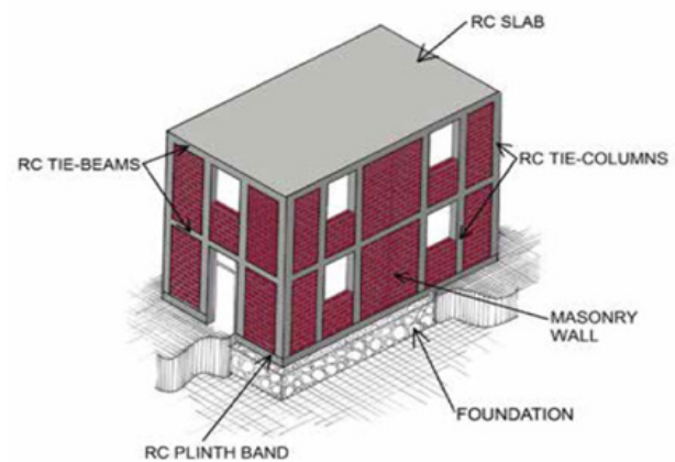
FIGURE 18: Component of confined masonry building
